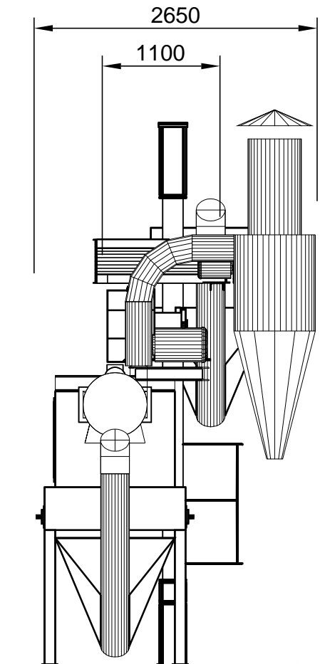
END VIEW
