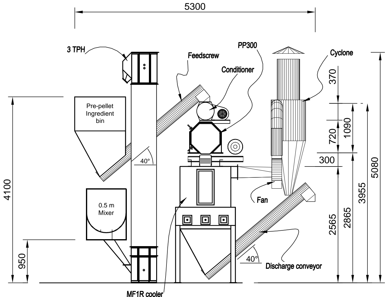
SIDE VIEW
